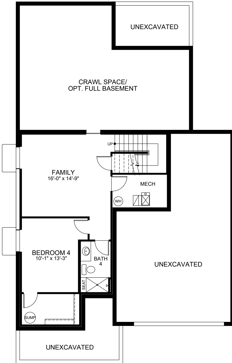
OPTIONAL PARTIAL FINISHED BASEMENT
