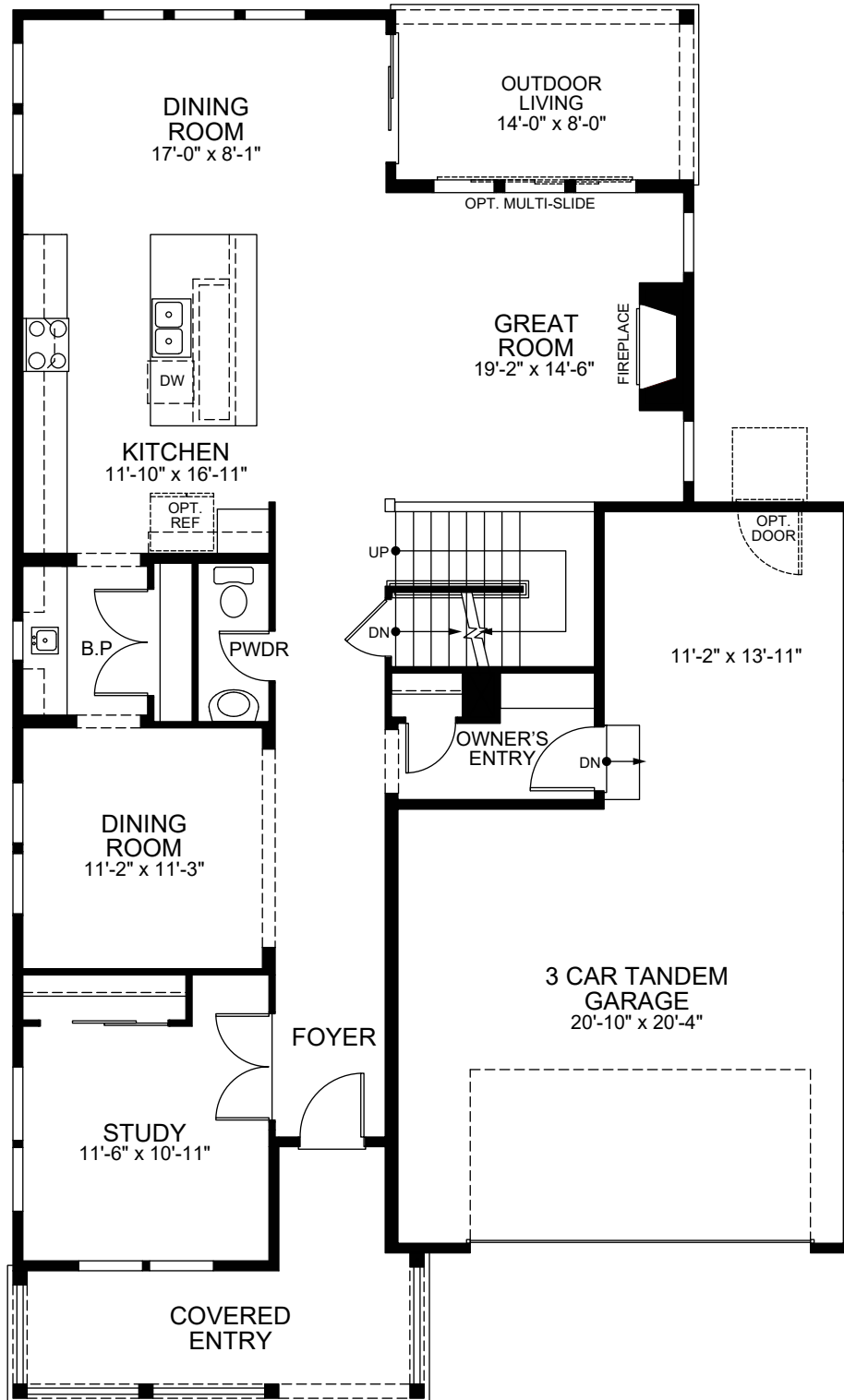
FIRST FLOOR
