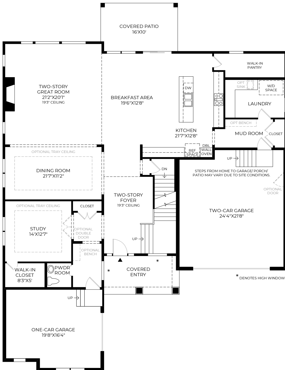
First Floor 9' CEILING HEIGHT
